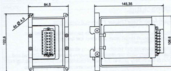
Fig. 4: C9900-U332_dimensions vertical mounting
