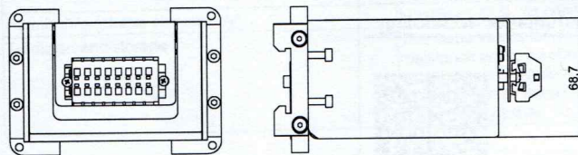
Fig. 5: C9900-U332_dimensions horizontal mounting
