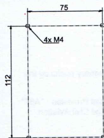
Fig. 6: C9900_U332_mounting without DIN rail
